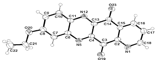
Figure 2. ORTEP drawing of 9b with an atomic labeling (the numbering scheme shown does not correspond to that of the IUPAC nomenclature).
