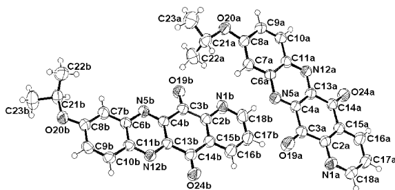
Figure 3. ORTEP drawing of 9c with an atomic labeling (the numbering scheme shown does not correspond to that of the IUPAC nomenclature).
